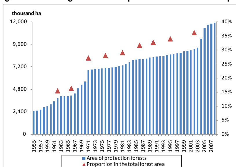
Figure 10: Change in area of protected forests of Japan
