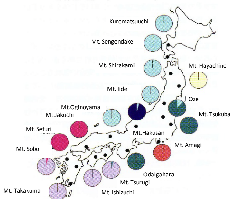
Figure 32: Variation of mitochondrion DNA of Japanese beech
