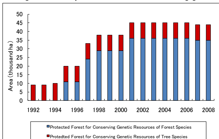
Figure 33: Change in area of protected forest for conserving genetic resources
