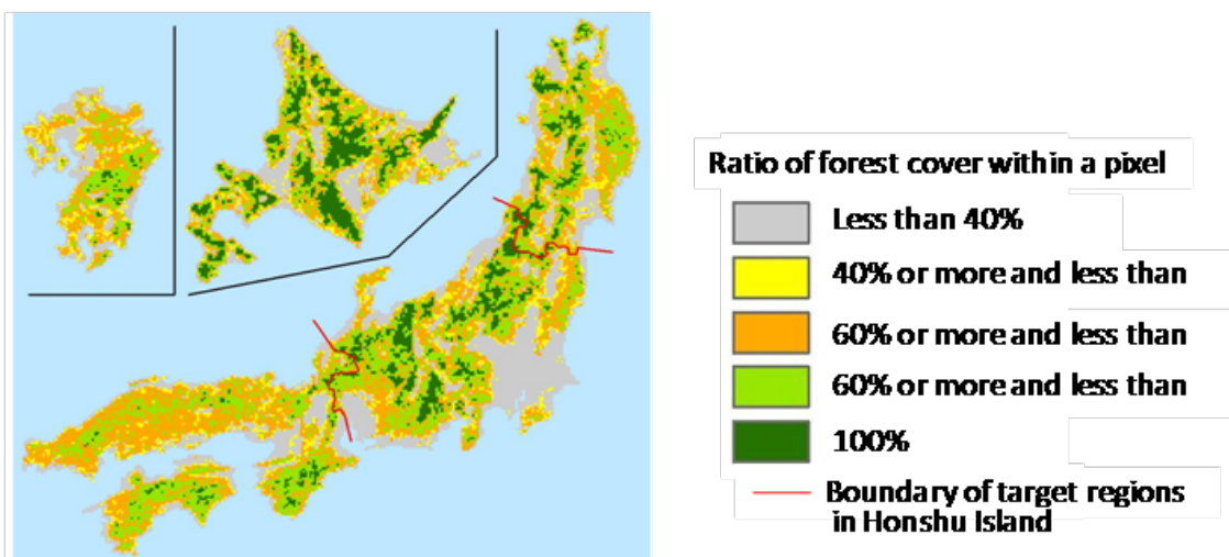
Figure 28: Distribution of forest cover rate in 4,000 x 4,000 meter pixels
