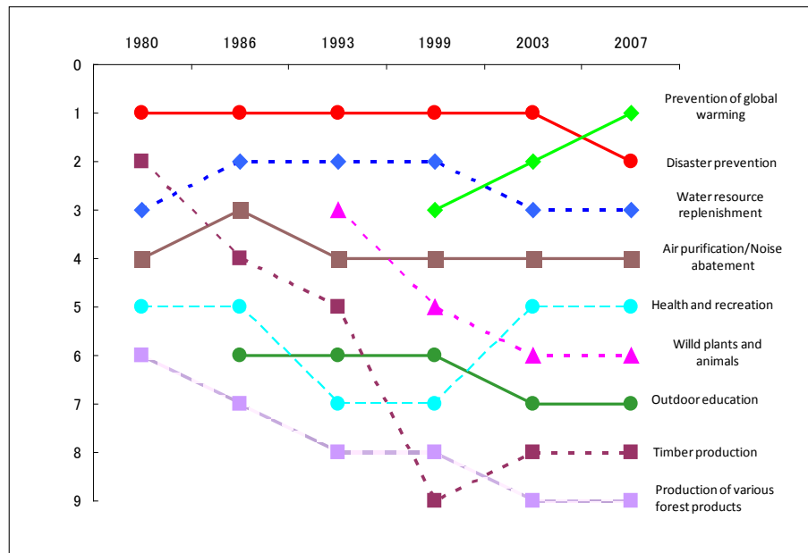
Figure 5: Change in Japanese People's Expectation to forest roles
