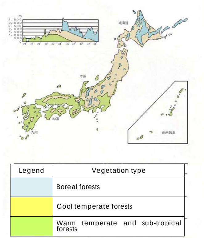
Figure 3: Distribution of forest types in Japan
