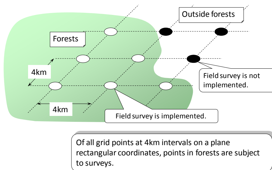
Figure 12: Structure of monitoring spot of Forest Resource Monitoring Survey of Japan
