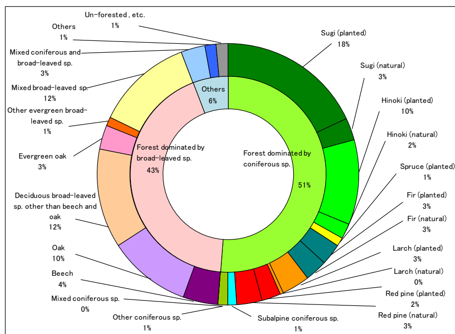
Figure 22: Composition of forest ecosystem types of Japan
