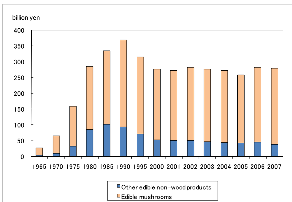
Figure 57: Change in the total production value of edible non-wood forest products
