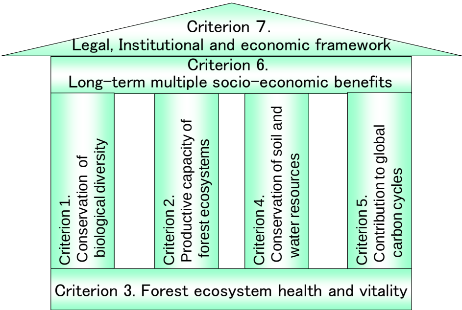
Figure 15: Conceptual structure of the Montreal Process criteria
