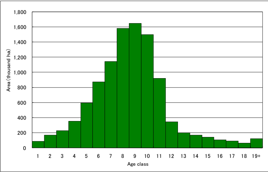
Figure 4: Distribution of age classes of planted forests of Japan
